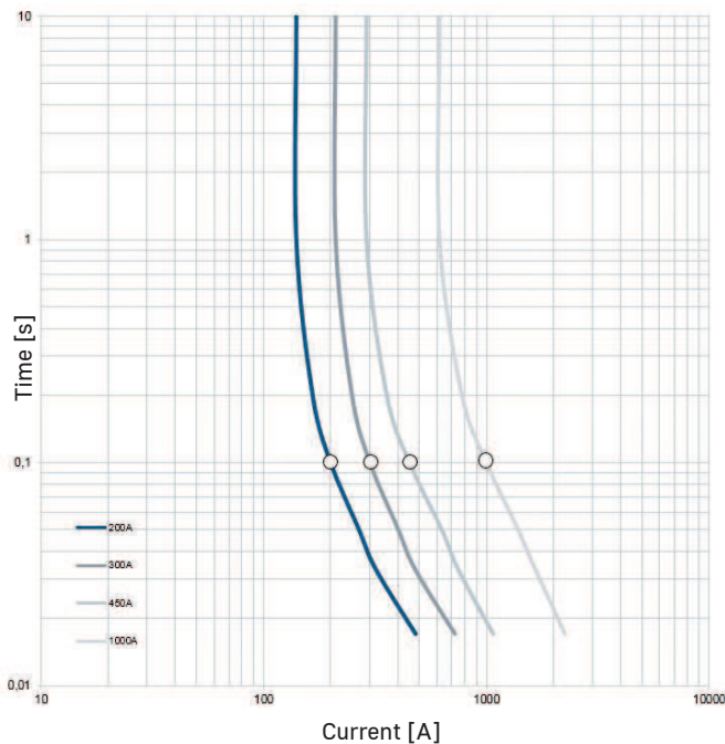
Current / time characteristic
