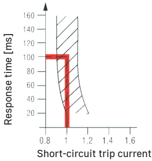
Response characteristic
