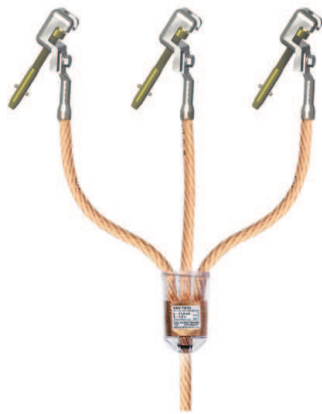
Line cables with ball tong
