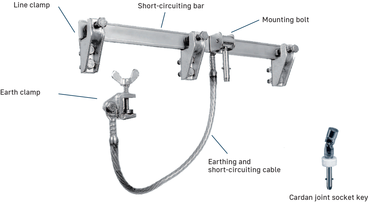
Short-circuiting bar with accessories
