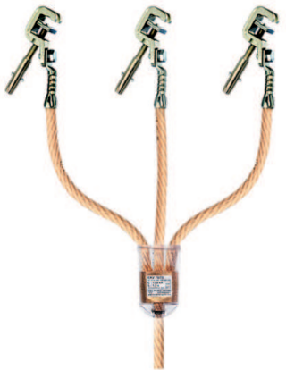
Line cables with universal line clamp
