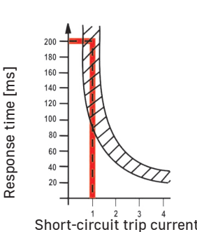
Response characteristic
