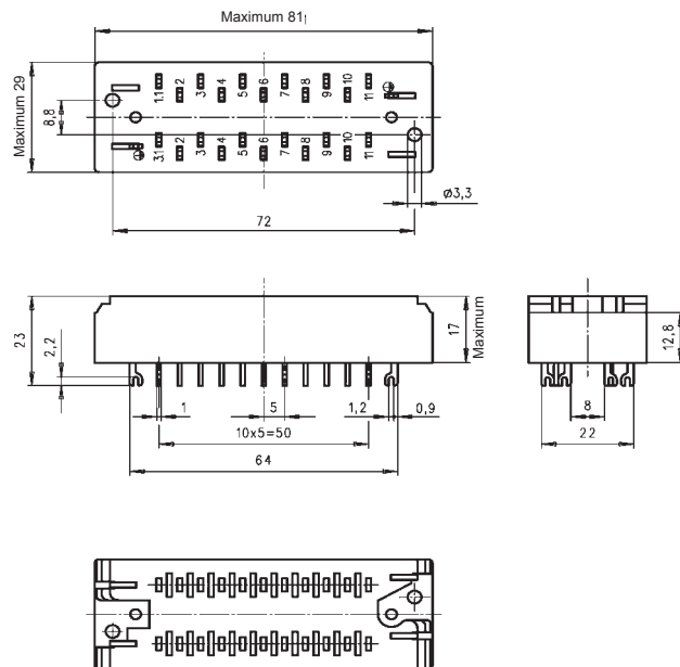
Dimensioned drawing Rs 805 202 Sheet 02; 22 poles
